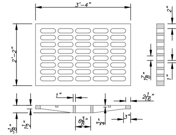
CAST IRON GRATING Traffic Bearing
