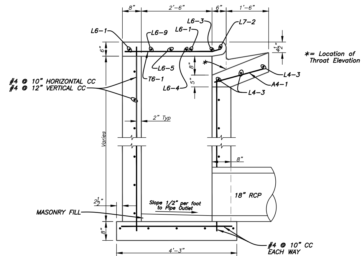
SECTION B-B
