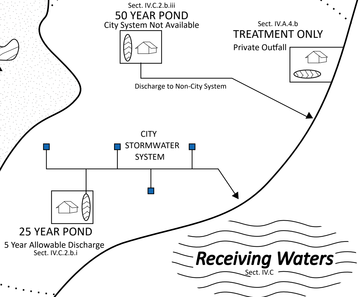
Figure 1 Stormwater Ponds Attenuation Criteria
