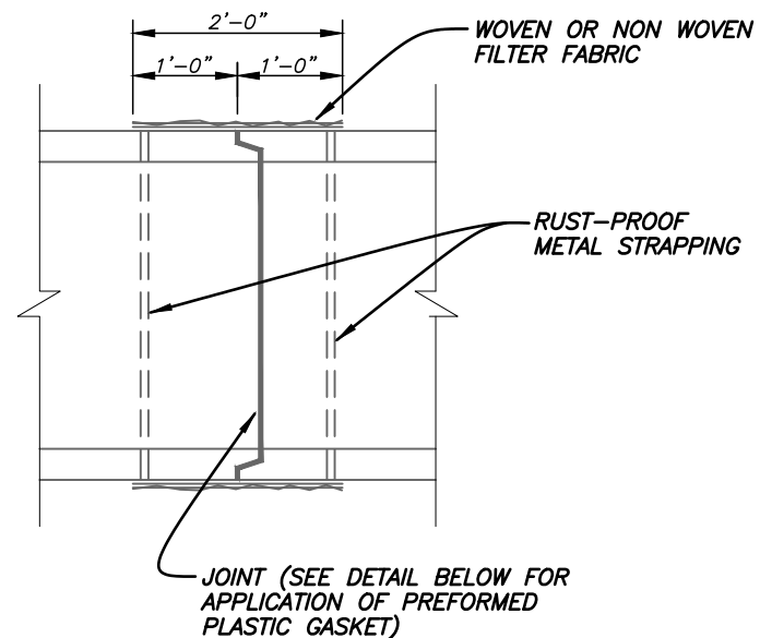
PIPE SECTION
