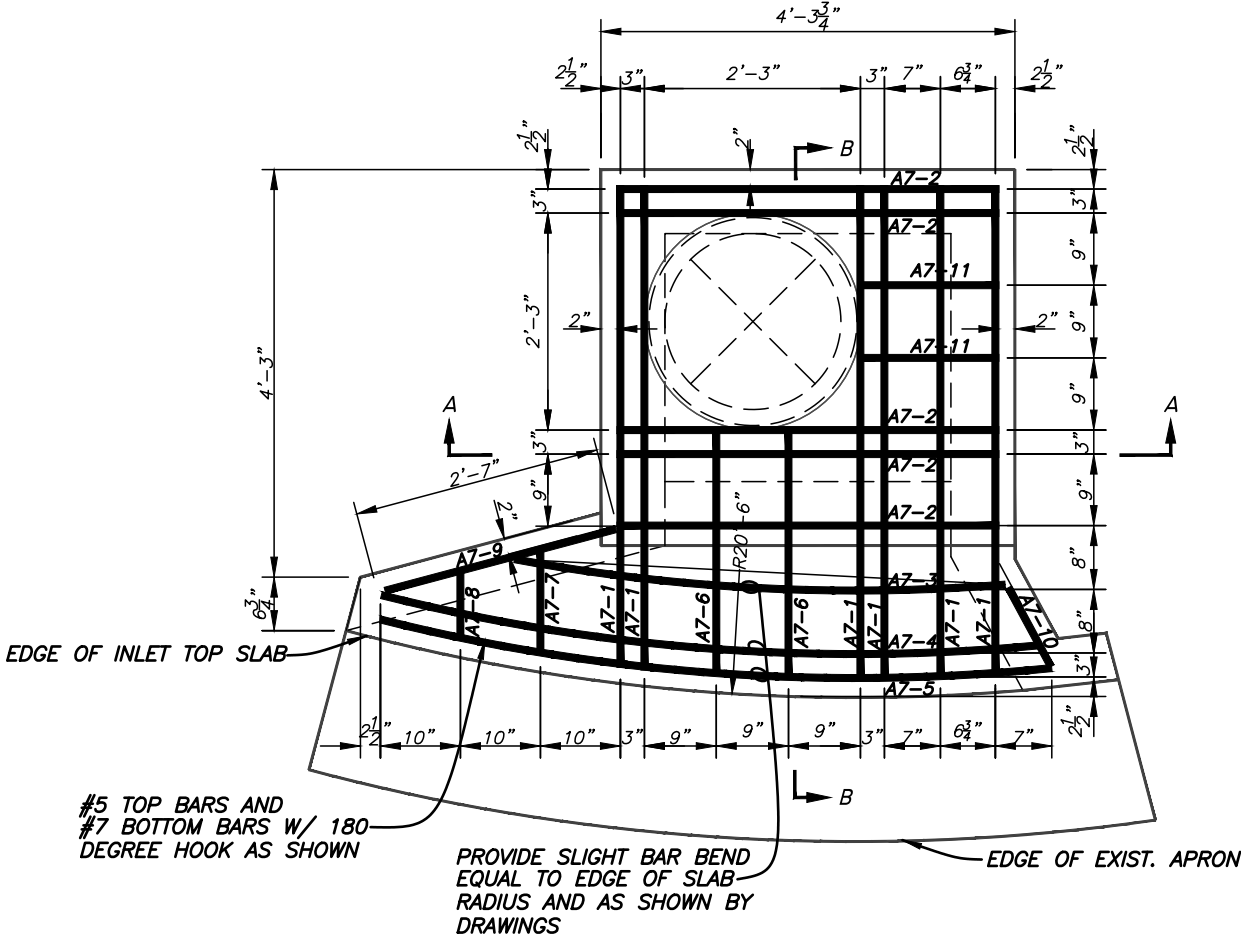
PLAN - NEW TOP SLAB REINFORCEMENT Scale: 1/2" = 1'-0" Note: ALL BARS SHALL HAVE 180 DEGREE HOOKS (TYPICAL)
