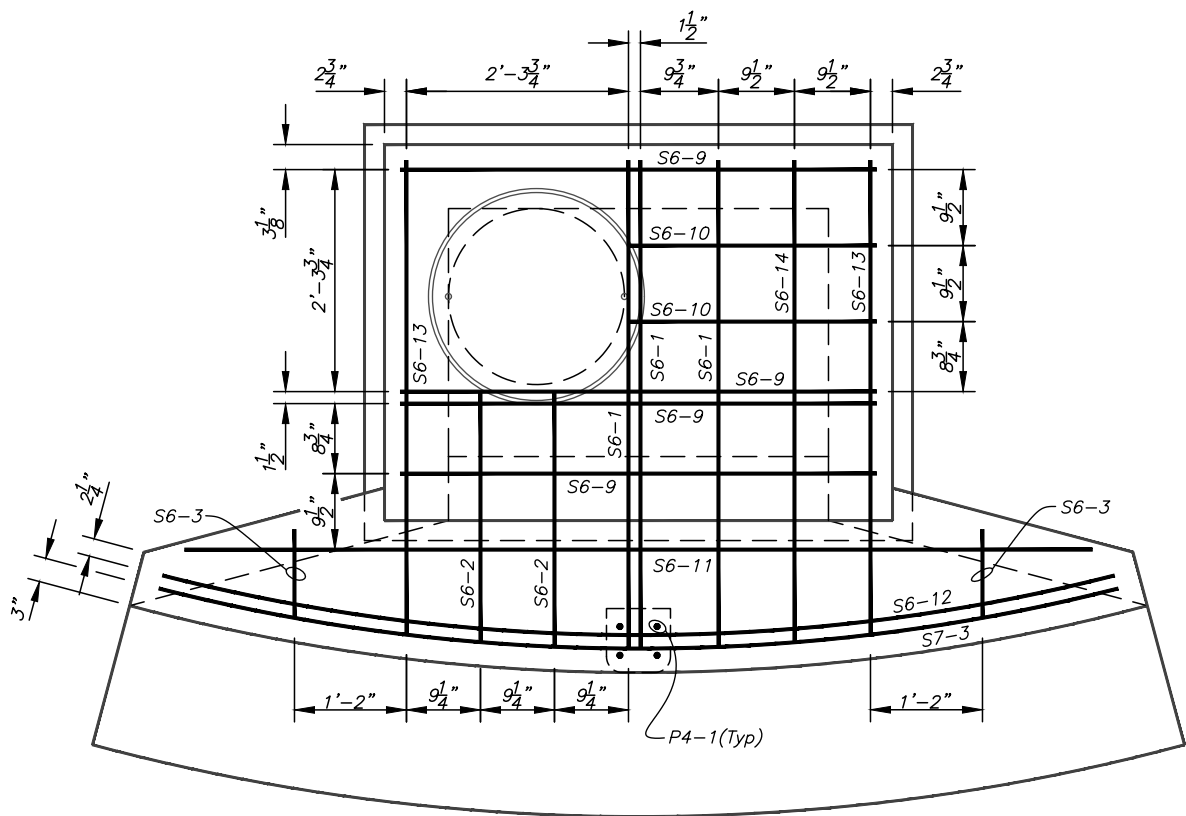
PLAN - TOP SLAB REINFORCEMENT Scale: 1/2" = 1'-0"
