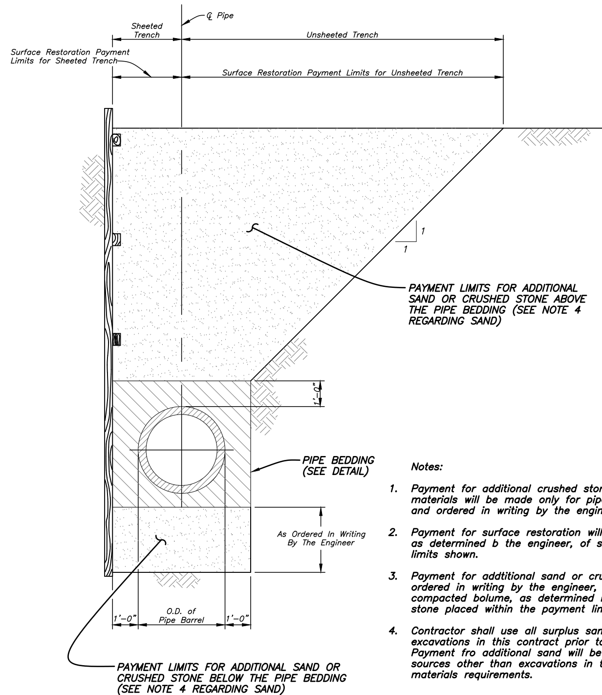
PAYMENT LIMITS FOR SURFACE RESTORATION AND ADDITIONAL SAND OR CRUSHED STONE FOR TRENCH STABILIZATION Not To Scale
